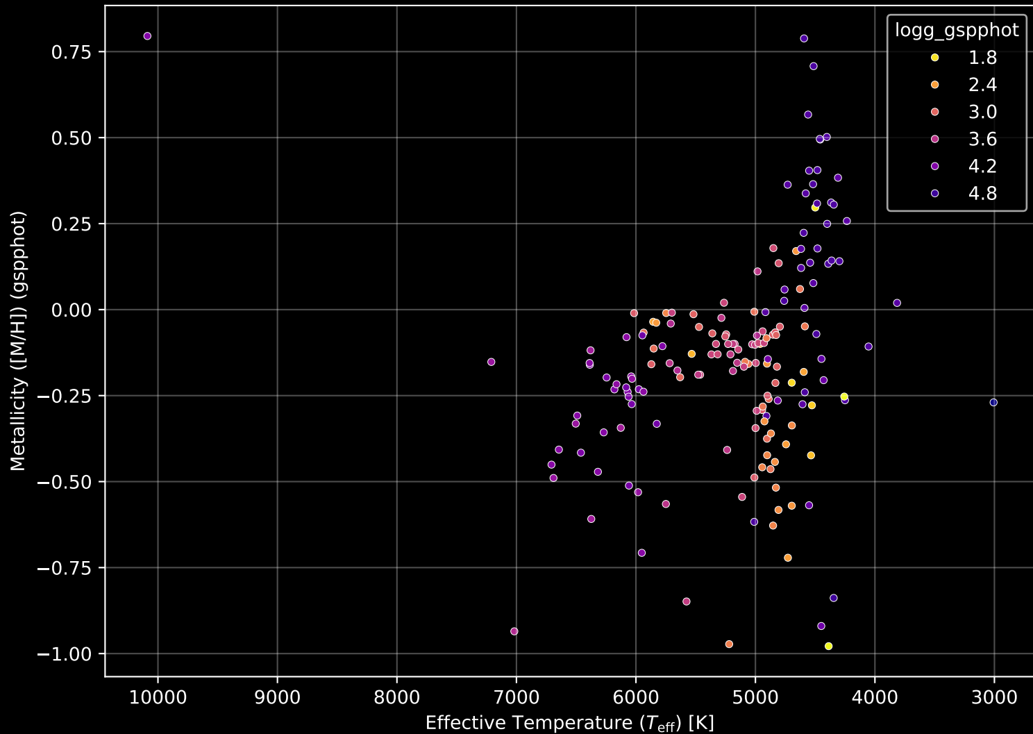
APOGEE DR17 Field: [070+54] Stellar Population Parameters (n= 171)
