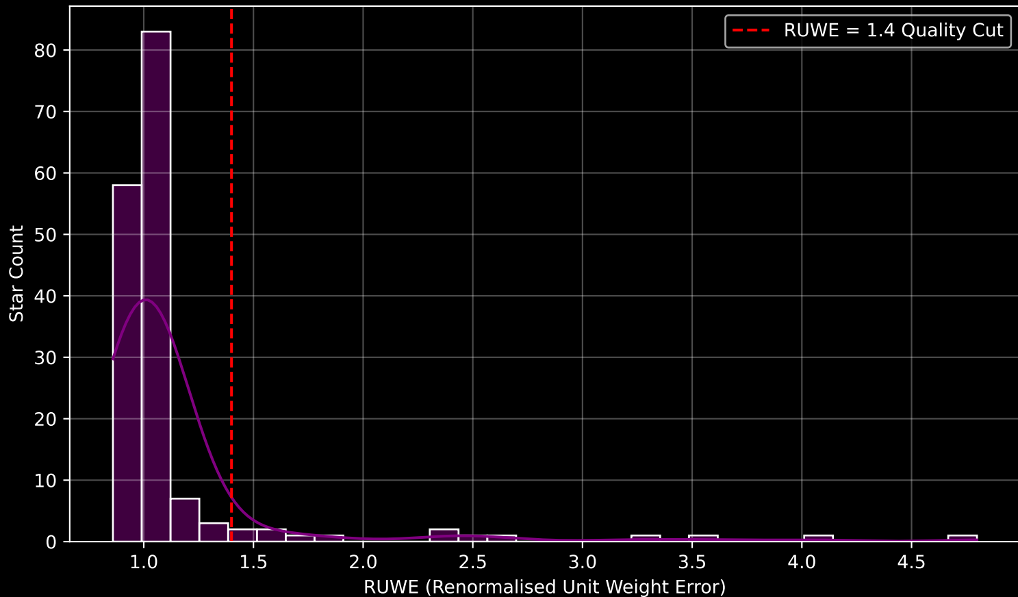
GAPOGEE DR17 Field [070+54] RUWE Distribution (n= 165)
