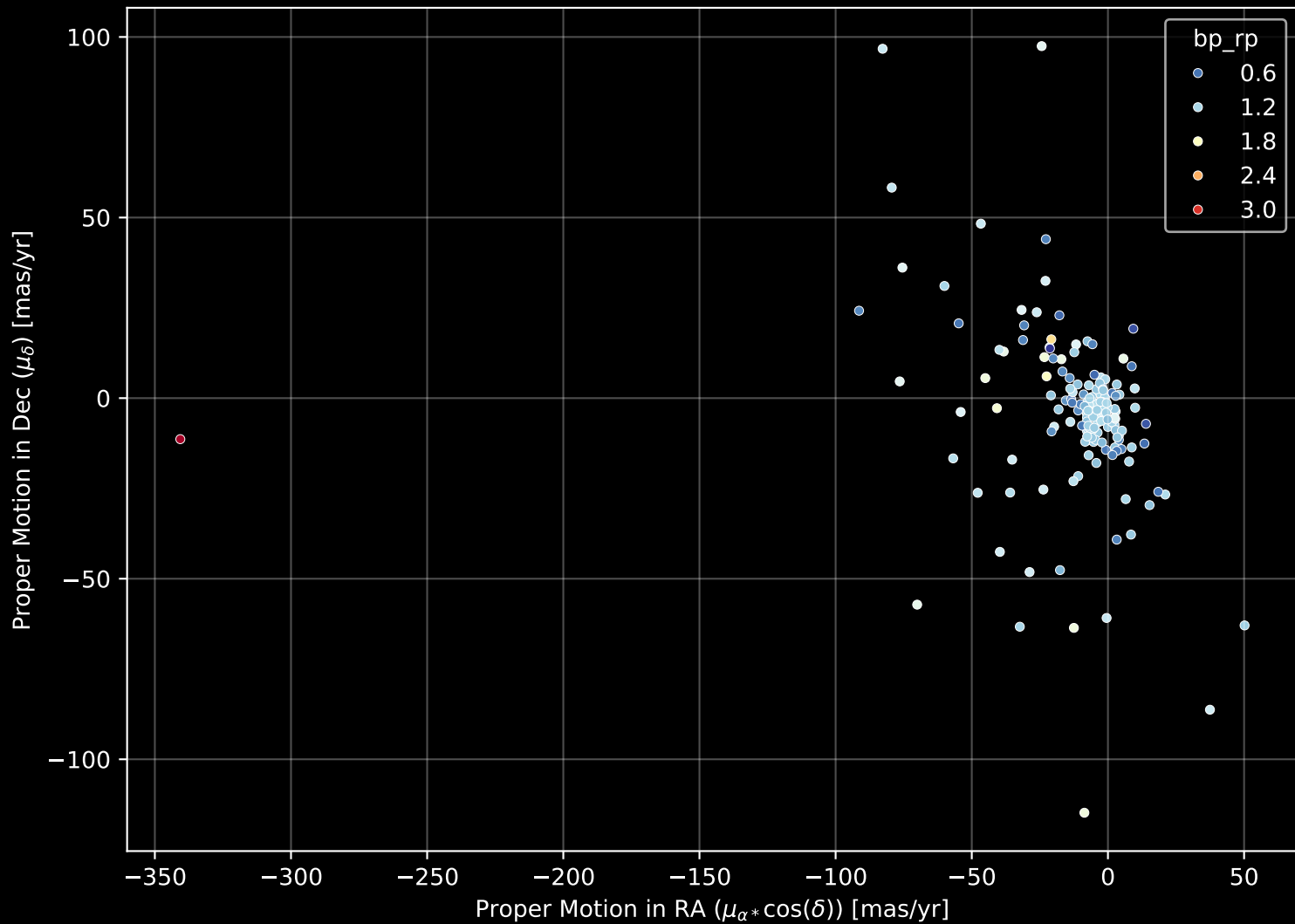
APOGEE DR17 Field: [070+54] Proper Motion Diagram (n= 171)
