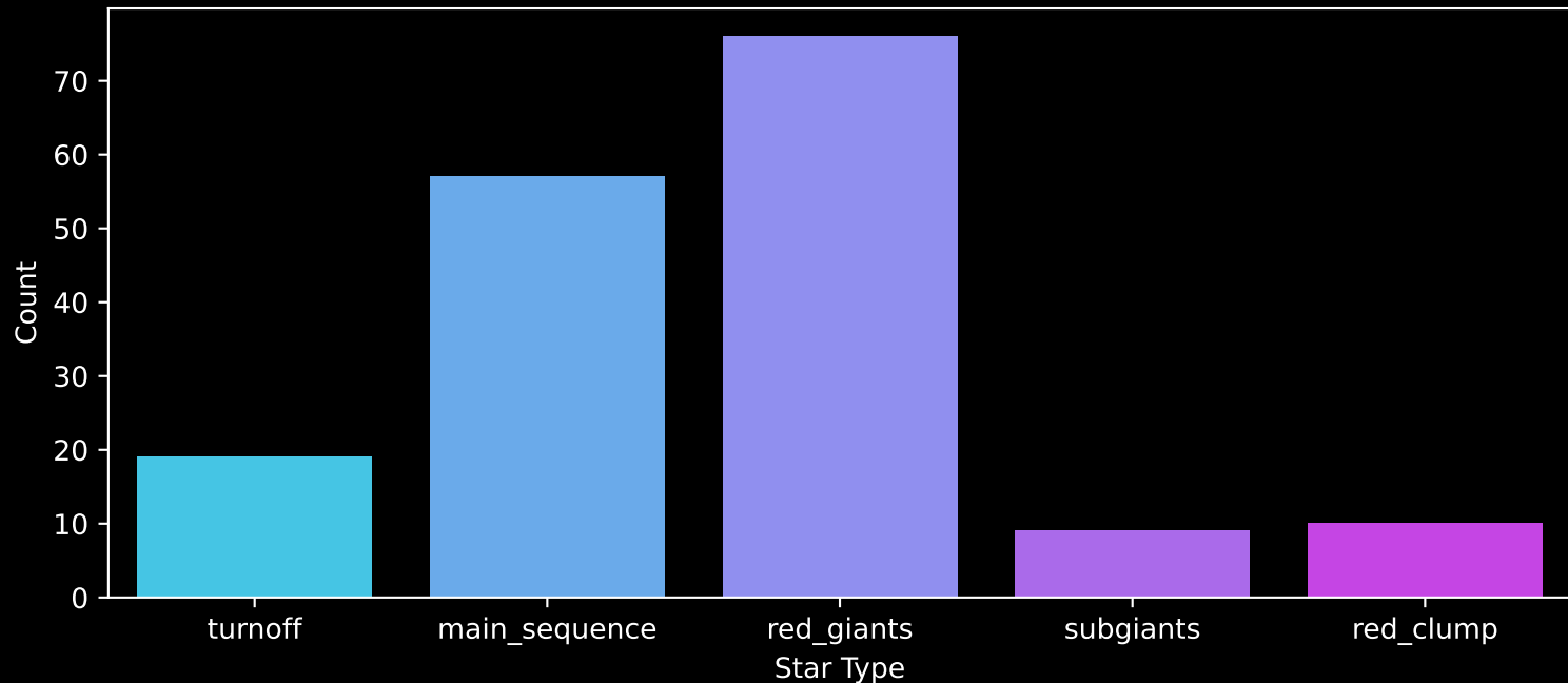
APOGEE DR17 Field: [070+54] Count plot of Star Type
