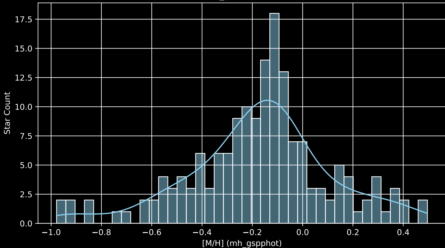
APOGEE DR17 Field: [070+54 [M/H] (mh_gspphot) (n= 166)
