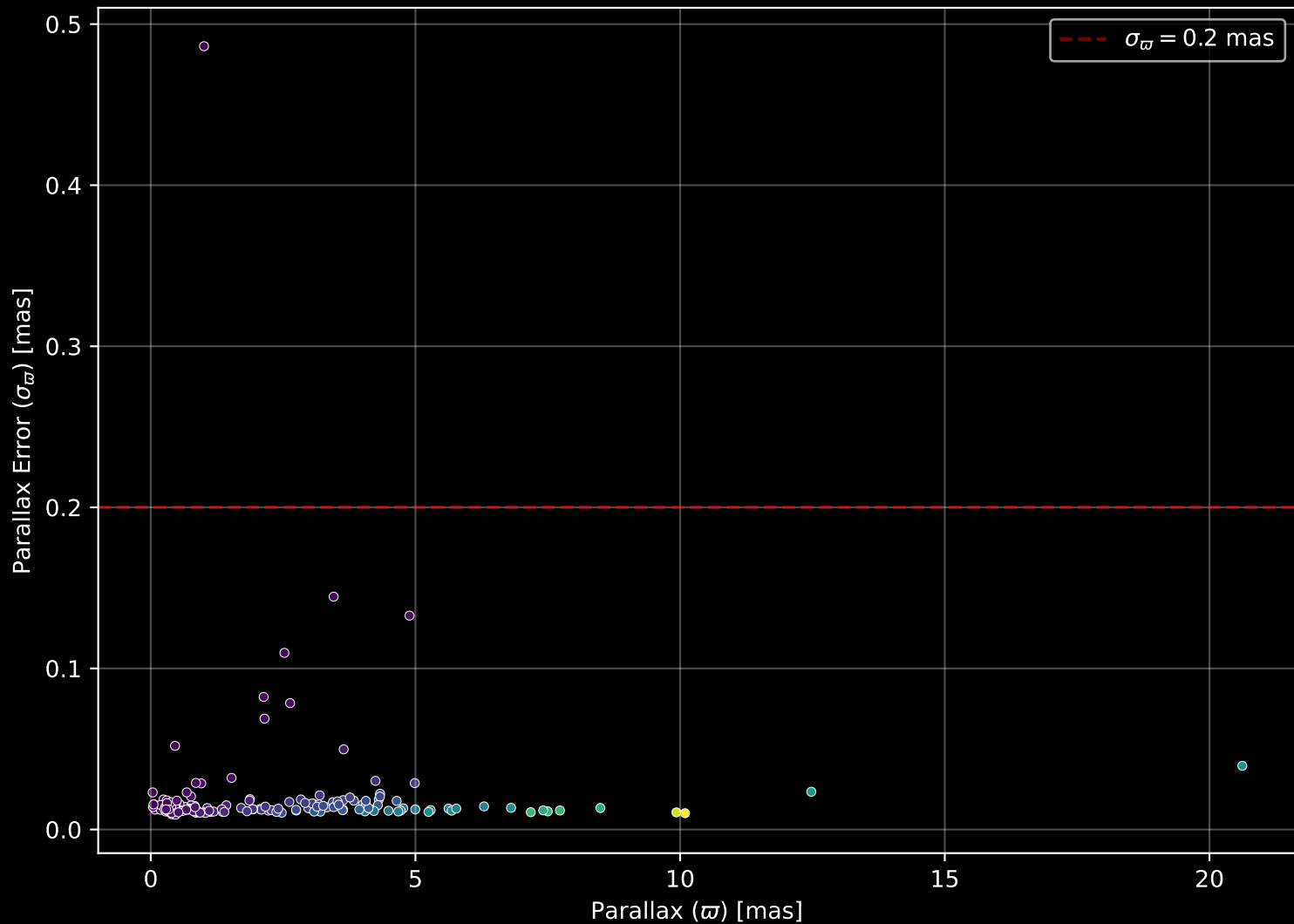
APOGEE DR17 Field: [070+54] Parallax Quality (n= 171)
